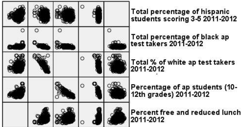
Figure 1. Scatterplots of the Variables
