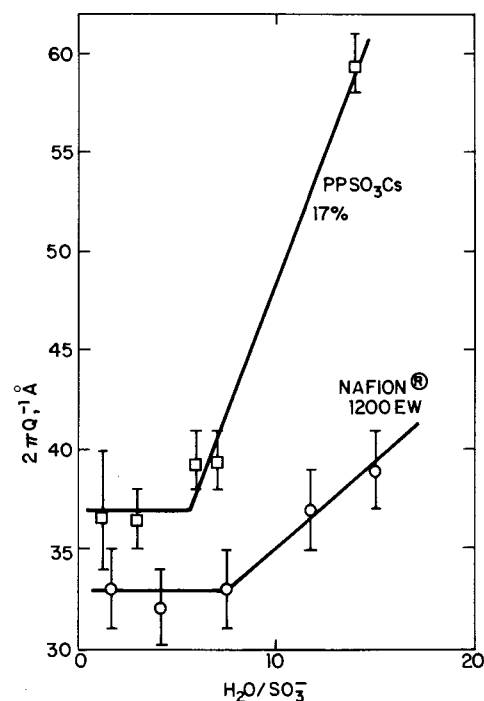
Figure 8. Bragg spacing of the SANS peak vs. waters per sulfonate groups for the 17% polypentenamer sulfonate ionomer and a 1200 equivalent weight Nafion membrane. The Nafion results are data from Roche et al. 16 used with permission.
