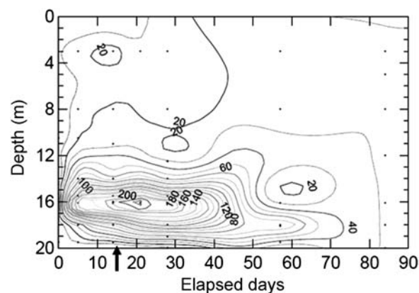
Fig. 2. Isopleths of seston \delta^{15}\text{N} (above background) sampled at four stations in Laguna El Tejo from 17 September to 10 December 1997. The isotope injection at 15.5 m occurred after background measurements were made on 17 September. The arrow on the x -axis shows the date when DVM measurements were made (30 September to 1 October).
