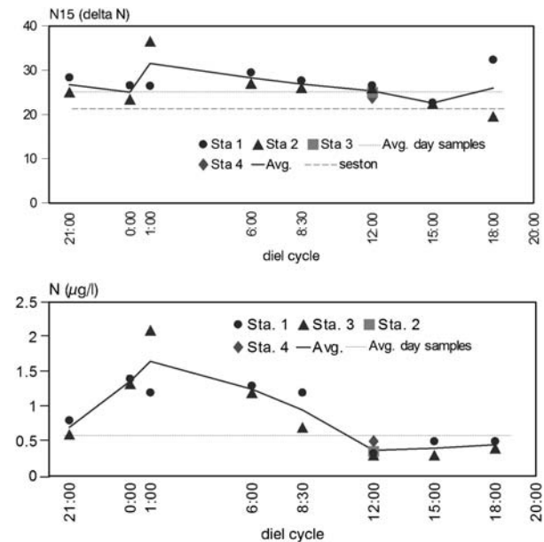
Fig. 5. (Upper) Diel changes in the isotopic signatures of zooplankton captured with vertical hauls (0–9 m) at different stations in the epilimnion of Laguna El Tejo on 30 September–1 October 1997. The bold dashed line shows the mean isotopic signature of seston in the epilimnion on this date. The light dashed line shows the mean isotopic signature of the day samples. (Lower) Changes in the nitrogen mass of zooplankton in the epilimnion of the lake over the diel cycle, light dashed line shows the mean nitrogen mass of the zooplankton day samples. Represented values at 0:00 h and 12:00 came from the series of samples taken with plankton traps. (delta N, \delta^{15}\text{N} ), mean isotopic signatures are expressed in ‰.
