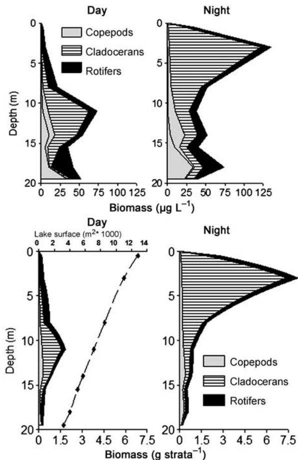
Fig. 4. (Upper) The vertical profile of the biomasses of different taxonomic groups in Laguna El Tejo on 1 October 1997. (Lower, left) The hypsographic curve of Laguna El Tejo showing the cross-sectional area at different depths, as well as the daytime whole lake estimates of integrated zooplankton biomass within different depth strata. (Lower, right) Night-time whole-lake distributions of different zooplankton taxa (g/strata). Distributions in the lower two figures are corrected for the relative lake volumes in each depth strata.
