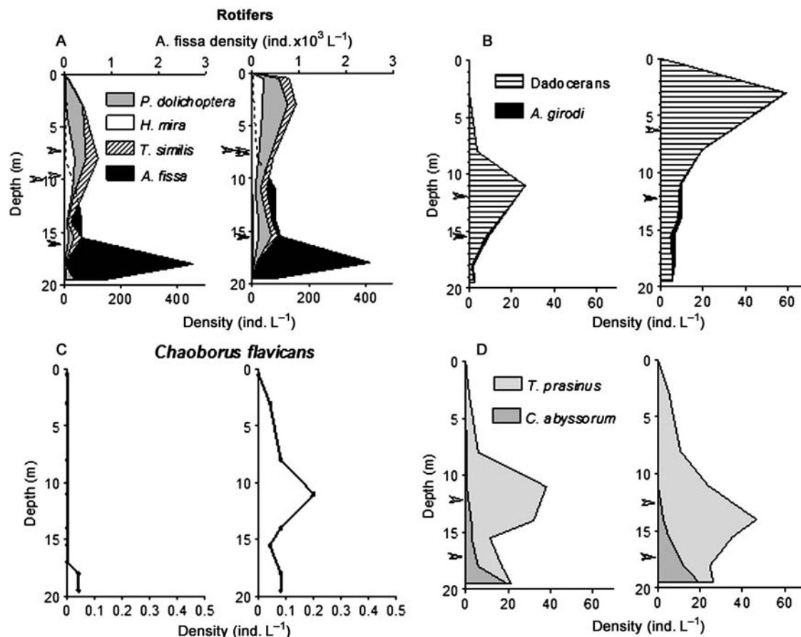
Fig. 3. Vertical distribution patterns of zooplankton in Laguna El Tejo on 1 October 1997. In each pair of figures, the daytime distribution is shown on the left and the night-time distribution on the right. Arrows show the MRD of each taxon (not shown for Chaoborus ).
