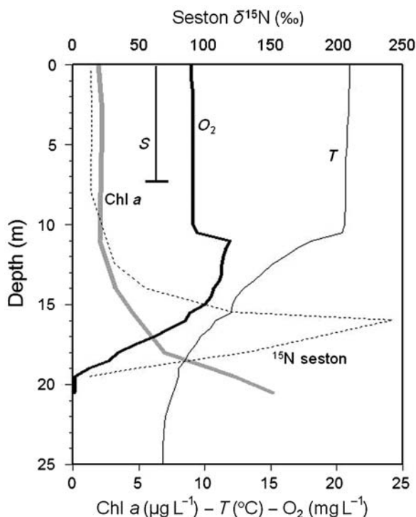
Fig. 1. Temperature ( T ), oxygen ( \text{O}_2 ), chlorophyll a and seston \delta^{15}\text{N} profiles in Laguna El Tejo on 30 September 1997. The Secchi ( S ) depth transparency is also shown.
