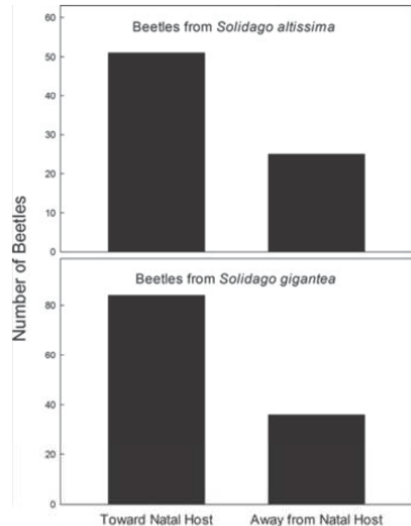
Fig. 1. Decisions of gall beetles when exposed to their natal host galls. The bars show the number of gall beetles that made each decision from the (top) Solidago altissima ( P < 0.001) and (bottom) S. gigantea ( P < 0.001) host-associated populations.
