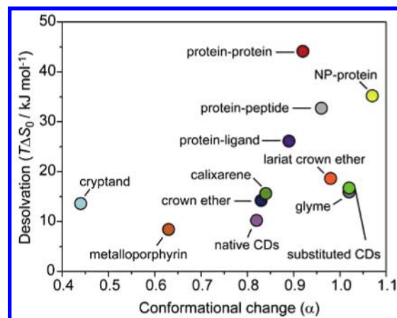
Figure 6. Slope ( \alpha ) and intercept ( T\Delta S_0 ) values for various host-guest systems. Protein-ligand interactions have been divided into protein-peptide and protein-other (protein-ligand) interactions.
