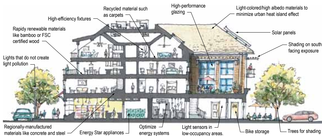
Section drawing illustrating sustainable building techniques.
