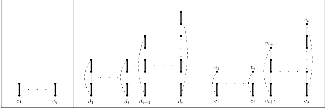
Figure 1: Components (paths or cycles) of G with edges in a maximum matching E' in bold.
