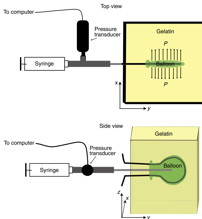
Fig. A2. Balloon pressure transducer setup. The balloon is stretched to a 2-D disk using a wire and is glued to the end of a tube (grey line), which is connected to a Luer lock adapter (thicker grey line). The adapter is connected to a syringe filled with water and a pressure transducer. The balloon, syringe and pressure transducer were held in the horizontal x - y plane, as shown in the top-view scheme, to minimize variations in pressure ( P ) with water height.
