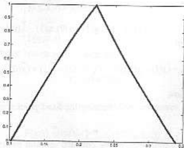
Figure 1 : First Solution of Fixed Point Method with x_0 = (0.210, 0.210, 0.109, 0.128) .
