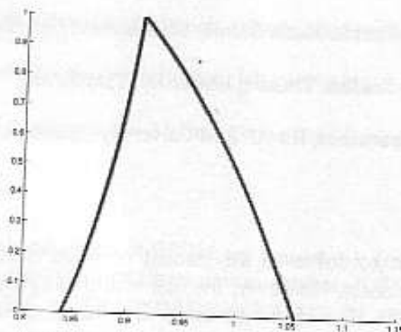
Figure 3: Positive Solution of Fixed Point Method with x_0 = (0.91, 0.91, 0.15, 0.15) .
