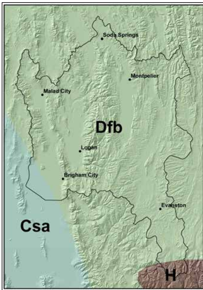
Figure 4.1 Climate types (Gabler et al., 1997)
