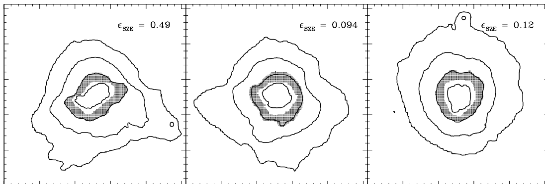
Figure 5. Sample of SZ decrement maps for a hydrodynamic simulation cluster. Each panel presents the map for a LOS along each of the axes of the simulation box. Each square is 2 h^{-1} Mpc across. The solid lines show contours of constant temperature decrement, spaced by factors of 3. The shaded area is the region used to calculate the ellipticity shown in the upper right corners (see text for discussion, and the Supplementary Material section for details of the full figure).
