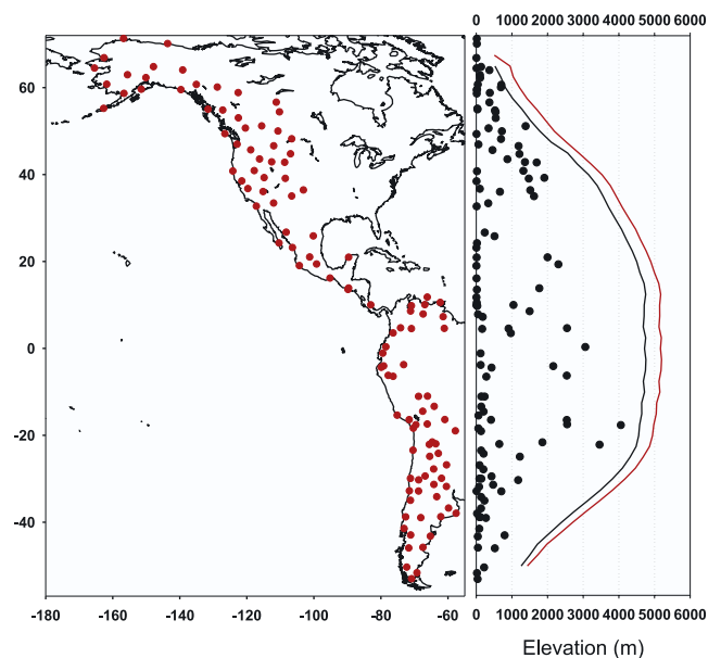
Figure 3. Distribution of planned GCOS surface station network in the western Americas and (on the right, black dots) the elevations of those stations with respect to latitude. Only 3 stations are planned for sites above 3000 m. Thus, the network fails to monitor those regions that model simulations indicate will have the greatest changes in temperature. Mean annual freezing level heights for control runs and 2\times \text{CO}_2 simulations are shown at right, in relation to the planned GCOS network.
