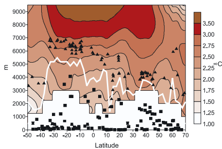
Figure 4. Mean annual change in temperature ( 2\times\text{CO}_2 minus control runs) for the 7 models listed in Table 1 compared to the planned GCOS surface network (squares) shown in Figure 3. More stations at higher elevations are needed to properly assess the model projections and monitor the large changes that the models indicate will affect high montane regions. The small black triangles represent the highest elevation mountains in countries along the transect.
