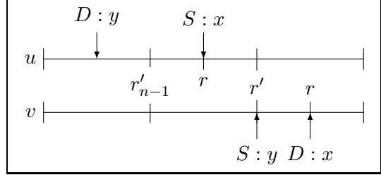
Figure 4: Two n -rankers appear in different order and r' ends with \triangleright .
