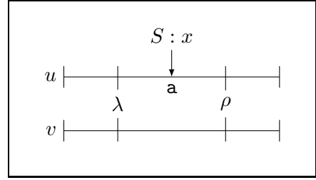
Figure 9: A letter occurs between rankers r, r' in u but not in v
