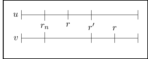
Figure 10: Ranker positions, case (4)
