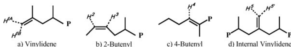
Figure 1. Proton numbering of unsaturated groups detected by ^1\text{H} NMR.
