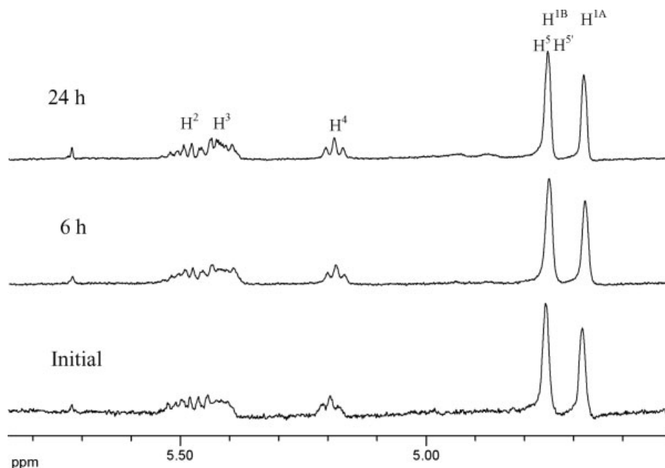
Figure 2. ^1\text{H} NMR olefinic region (400 MHz, \text{TCE-}d_2 , 100\text{ }^\circ\text{C} , reference \text{C}_2\text{HDCl}_4 at 5.95 ppm) of iPP during the isomerization reaction.
