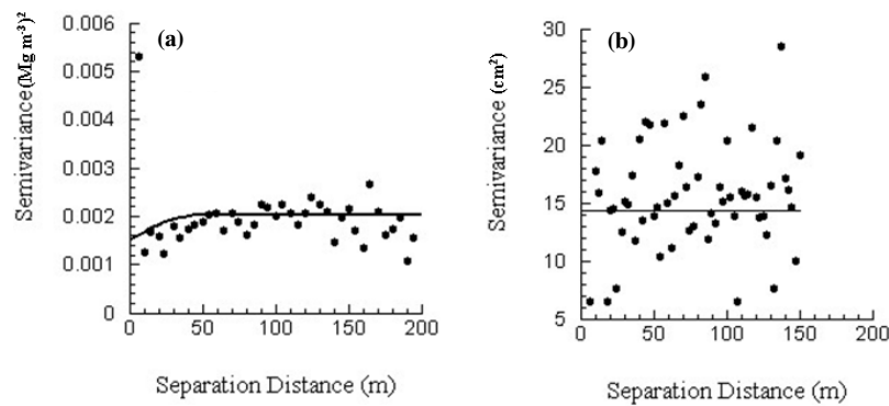
Figure 6. Semivariances for (a) maximum bulk density with theoretical exponential semivariogram model fit and (b) depth to maximum bulk density with pure nugget semivariogram model fit.
