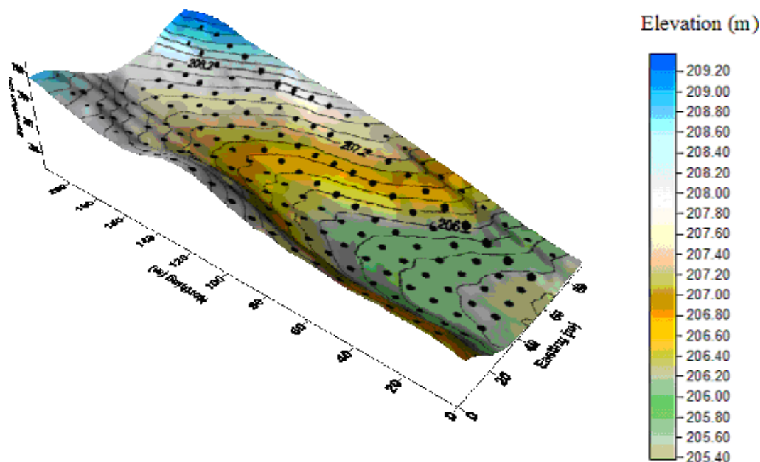
Figure 1. Elevation of the sampling field of Pacolet sandy loam soil. Dots indicate the sampling points for cone index measurement.
