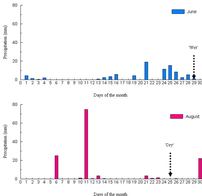
Figure 2. Precipitation data for June 2004 (wet measurement date) and August 2004 (dry measurement date) for Auburn, Alabama.
