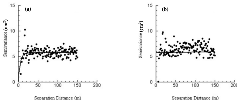
Figure 9. Semivariances for the depth to peak cone index and exponential theoretical model fit and pure nugget model fit for the measurement dates of (a) 29 June 2004 and (b) 25 August 2004.
