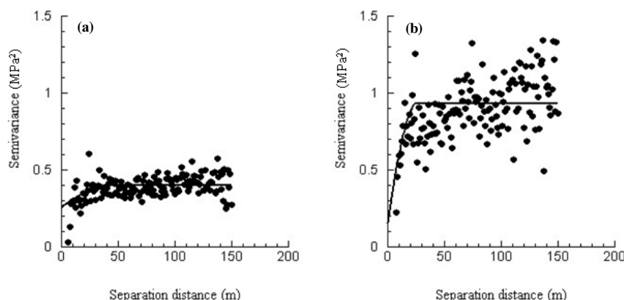
Figure 8. Semivariances for the peak cone index and spherical theoretical model fits for the two measurement dates of (a) 29 June 2004 and (b) 25 August 2004.
