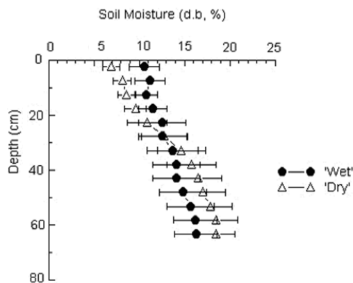
Figure 3. Soil moisture profile for the two measurement dates of 29 June 2004 (wet) and 25 August 2004 (dry). The horizontal bars indicate standard deviations.
