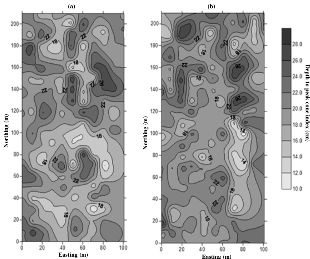
Figure 10. Contour map of the depth to peak cone index on Pacolet sandy loam soil for the two measurement dates of (a) 29 June 2004 and (b) 25 August 2004.
