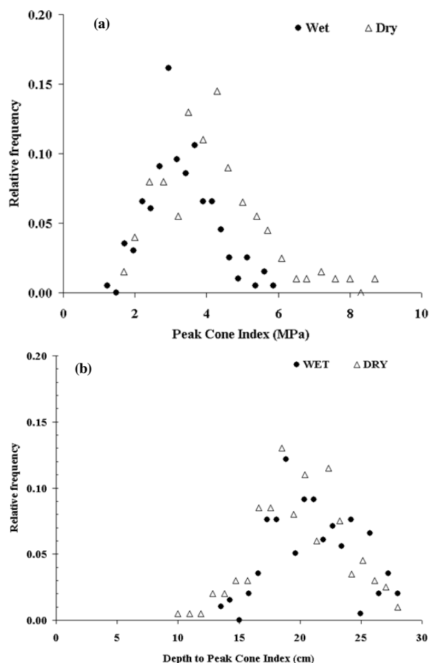
Figure 5. Relative frequency distribution of (a) peak cone index (MPa) and (b) depth to peak cone index for the two measurement dates of 29 June 2004 (circles) and 25 August 2004 (triangles).
