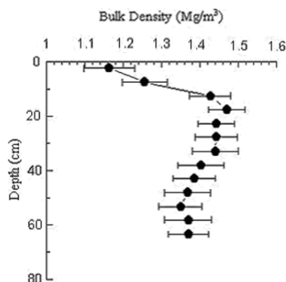
Figure 4. Bulk density profile averaged over the two measurement dates of 29 June and 25 August 2004. The horizontal bars indicate standard deviations.
