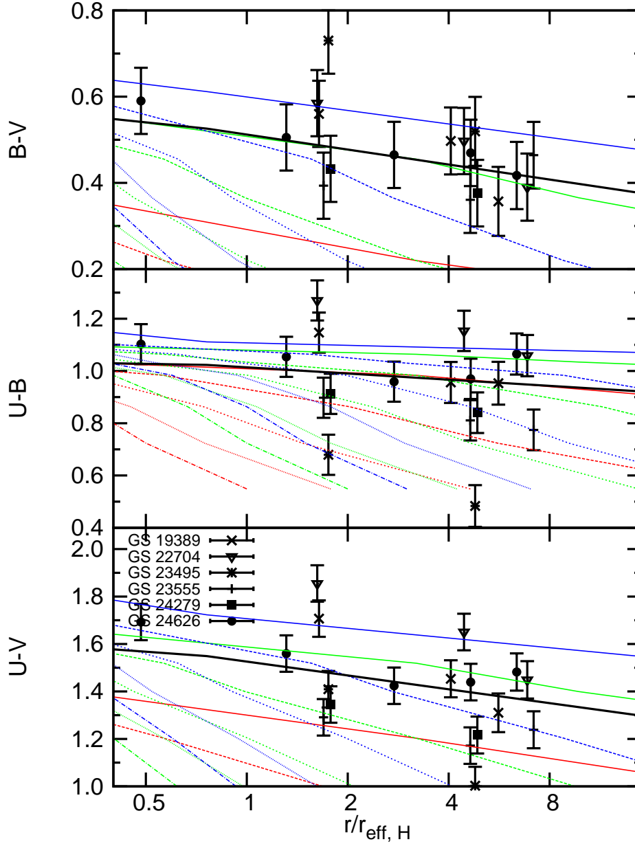
Fig. 7.— The predicted rest-frame ( B-V ), ( U-B ) and ( U-V ) color gradients from single stellar population models if the age of the dominant stellar population is the only parameter that varies as a function of radius in the galaxies (thin lines). The observed colors are plotted as black symbols with error bars. We only plot the predictions for the case of solar metallicity and zero dust extinction in this figure. Blue, green and red lines show the models in which the age at the center has been set at 3, 2 and 1 Gyr, respectively. For each color, different line patterns show different age gradients models, i.e., from top to bottom, \Delta \log(\text{age}) / \Delta \log(R/R_{\text{eff}}) = -0.2 (solid), -0.4 (long dashed), -0.6 (short dashed), -0.8 (dotted) and -1.0 (dashed-dotted). The thick black line shows the prediction of age gradient that best reproduces the observations. See the text for details.
