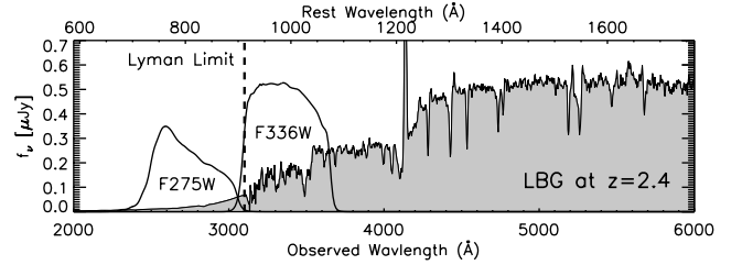
Figure 9. The composite LBG spectrum of Shapley et al. (2003) is shifted to z = 2.4 (the spectrum at \lambda_{\text{rest}} < 912 \text{ Å} is an estimate). Overplotted (with arbitrary scaling) are the transmission curves of the UVIS filters being used in the GOODS-N CVZ day-side observations. At z > 2.38 , the Lyman limit shifts redward of any significant transmission in the F275W filter. Therefore, this filter will probe the escaping Lyman continuum radiation for galaxies at 2.38 < z < 2.55 (where the upper limit is dictated by IGM opacity). Also demonstrated is the ability to efficiently select star-forming galaxies via a decrement in the F275W flux due to Lyman continuum opacity from H I in both the IGM and the interstellar medium of the galaxy (see text for details).
