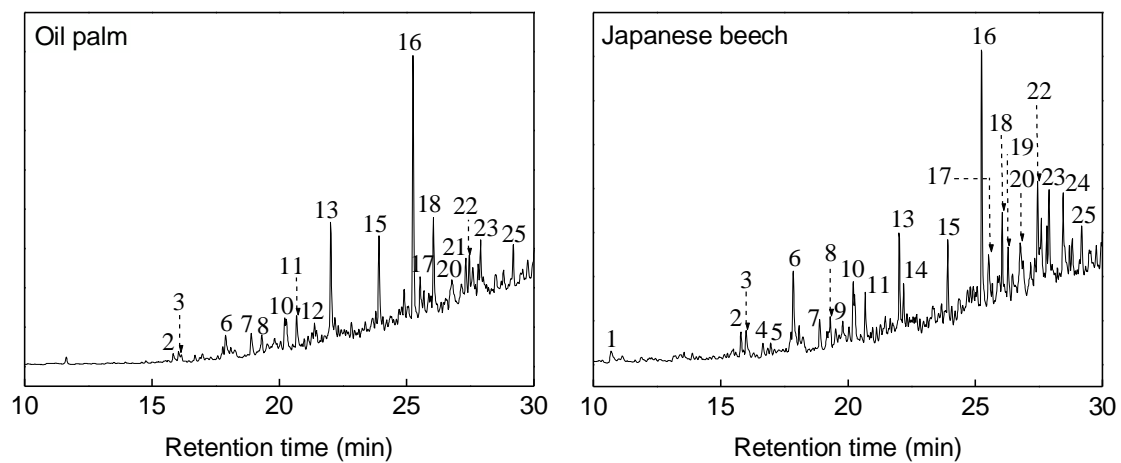
Figure 1 Total-ion chromatograms for the methanol-soluble portion from oil palm and Japanese beech in GC-MS analysis.
