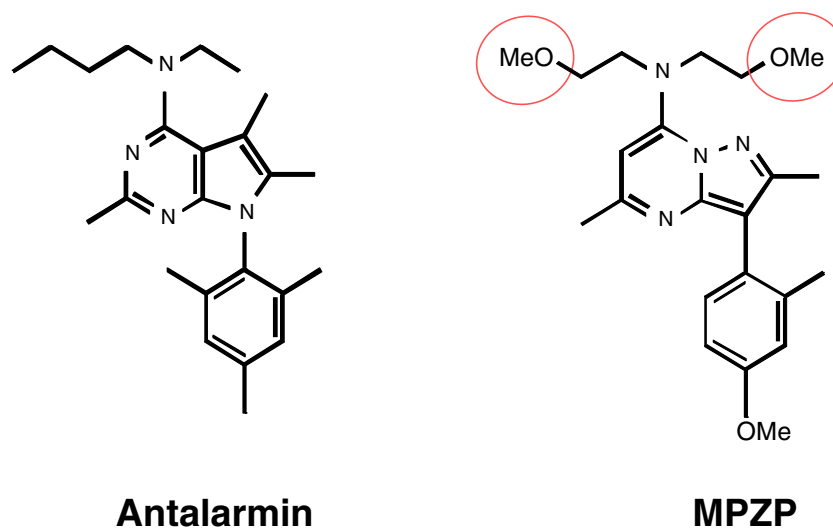
Fig. 1 Chemical structures of antalarmin and MPZP
