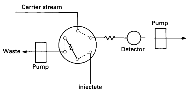
Fig. 1. Manifold and valve configuration used for time-based injections
