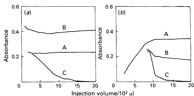
Fig. 4. Effect of injection volume on the height and integrity of the front and rear peaks for (a) \text{IO}_3^- \text{I}^- < \text{H}^+ < \text{IO}_3^- \text{I}^- (system 1a) and (b) \text{H}^+ < \text{IO}_3^- \text{I}^- < \text{H}^+ (system 1b). Height ( i.e. , absorbance) of A, front peak; B, rear peak; and C, valley between the peaks. Slug injection: flow-rate, 5 \text{ ml min}^{-1} ; \text{IO}_3^- \text{I}^- solution, 6.67 \times 10^{-6} \text{ M} in \text{KIO}_3 , 1.4 \times 10^{-2} \text{ M} in \text{KI} and 2 \times 10^{-3} \text{ M} in \text{NaOH} ; \text{H}^+ solution, 0.1 \text{ M} \text{HCl}
