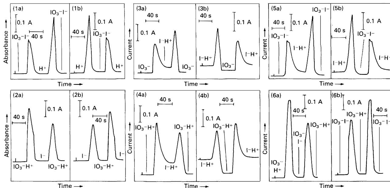
Fig. 3. Signals obtained with time-based injections for different systems. The signals are numbered according to the information given in Table 1. The experimental conditions are described in the text. Flow-rate, 2 \text{ ml min}^{-1} ; injection time, 1 min. Iodate, iodide and hydrochloric acid solution concentrations, 6.67 \times 10^{-6} \text{ M} , 0.23% and 0.1 M, respectively; non-acidic solutions were adjusted to pH 11.0 with sodium hydroxide solution
