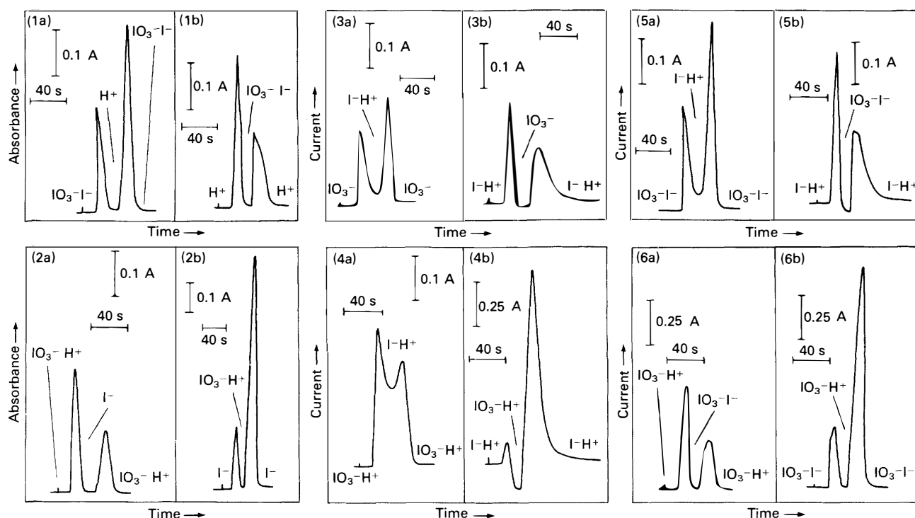
Fig. 2. Signals obtained with slug injections for different systems. The signals are numbered according to the information given in Table 1. Experimental conditions are given in the text. Flow-rate, 5 \text{ ml min}^{-1} . Iodate, iodide and hydrochloric acid solution concentrations, 6.67 \times 10^{-6} \text{ M} , 0.23% and 0.1 M, respectively; non-acidic solutions were adjusted to pH 11.0 with sodium hydroxide solution
