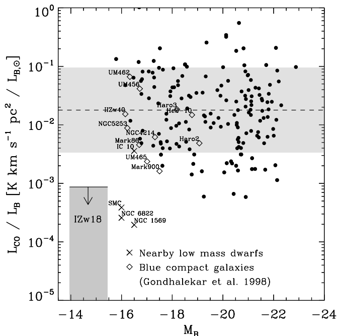
FIG. 3.—Plot of CO luminosity normalized by absolute blue magnitude for galaxies with Hubble type Sb or later (circles; Young et al. 1995; Elfhag et al. 1996; Böker et al. 2003; Leroy et al. 2005). We also plot nearby dwarfs from Table 1 (crosses) and blue compact galaxies compiled by Gondhalekar et al. (1998; diamonds). The dark shaded region shows our upper limit for I Zw 18, with the range in M_B for distances from 10 to 20 Mpc. The dashed line and light shaded region show the median value and 1\sigma scatter in L_{CO}/L_B for spirals and dwarf starbursts. Methodology: We extrapolate from I_{CO} in central pointings to L_{CO} assuming the CO to have an exponential profile with scale length 0.1 d_{25} (Young et al. 1995), including only galaxies where the central pointing measures >20\% of L_{CO} . We adopt B magnitudes (corrected for internal and Galactic extinction), distances (Tully-Fisher when available, otherwise Virgocentric flow corrected Hubble flow), and radii from LEDA (Lyon-Meudon Extragalactic Database; Paturel et al. 2003).
