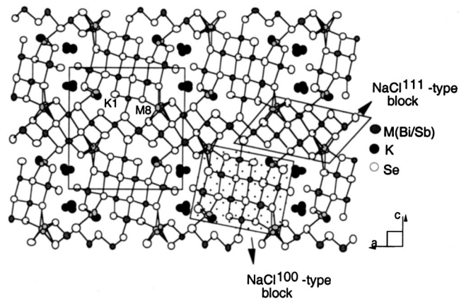
FIG. 3. The crystal structure of K_2Bi_{8-x}Sb_xSe_{13} ( x=4.0 and 2.4 ) with atom labeling showing the K1 and M8 sites. These sites are the first to be substituted with Sb.
