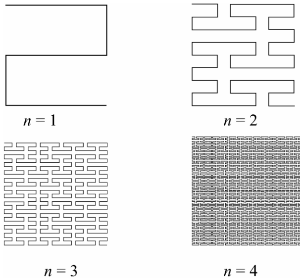
Fig.1. The First Four Iteration Levels to Generate the Peano Pre-Fractal Curve.
