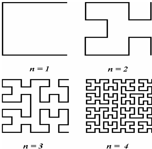
Fig.2. The First Four Iteration Levels to Generate the Hilbert Pre-Fractal Curve.
