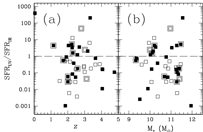
Figure 10. The ratio of SFR derived from the rest-frame UV ( SFR_{UV} ) and the rest-frame IR ( SFR_{IR} ) as a function of (a) redshift and (b) stellar mass ( M_* ). Galaxies with spec- z (photo- z ) are shown in filled (empty) symbols, and those detected by the Chandra in the X-ray are identified with a larger square. The dashed line marks the SFR_{UV} = SFR_{IR} relation.
