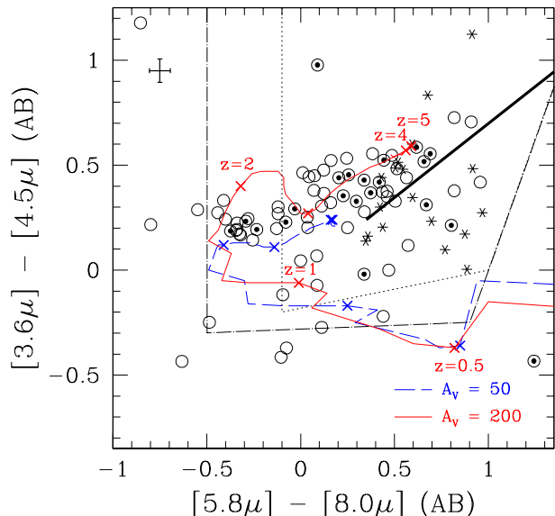
Figure 13. A [3.6\mu] - [4.5\mu] versus [5.8\mu] - [8.0\mu] IRAC color diagnostic diagram for heavily obscured starbursts and AGNs based on the color combinations proposed by Stern et al. (2005), adopted from Fig. 2 by Yun et al. (2008). All symbols and models shown are identical to those in Fig. 12.
