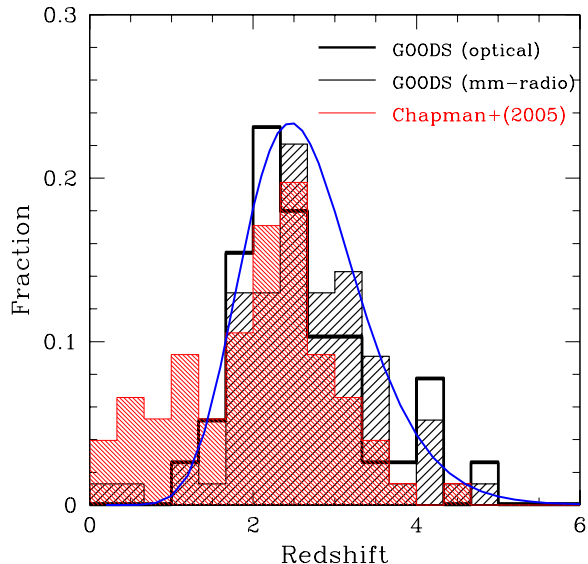
Figure 4. Redshift distributions of AzTEC sources in both GOODS fields based on the optical photoz ( z_{opt} , N = 38 ; blank histogram) and the millimetric photoz ( z_{MR} , N = 74 ; hatched histogram) are compared with that of the 76 radio-identified SCUBA sources with spectroscopic redshifts by Chapman et al. (2005, shaded histogram). The solid blue curve shown is a log-normal distribution as a function of (1+z) with a mean redshift of z_{\mu} = 2.6 and \sigma = 0.2 .
