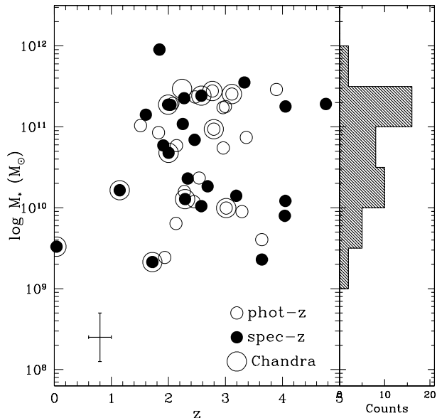
Figure 8. The stellar masses of AzTEC counterparts derived from optical and NIR photometry as a function of redshift. A histogram of stellar masses is shown on the right panel. Sources with a spectroscopic redshift are shown as solid symbols while the ones with a photometric redshift are shown as empty circles, and they represent similar ranges of stellar mass. Typical uncertainties for the M_* and photo- z estimates are shown on the bottom left corner. Those detected by the Chandra in the X-ray are identified with a larger circle. Only GOODS TFIT catalog sources with a proper stellar mass estimate are included.
