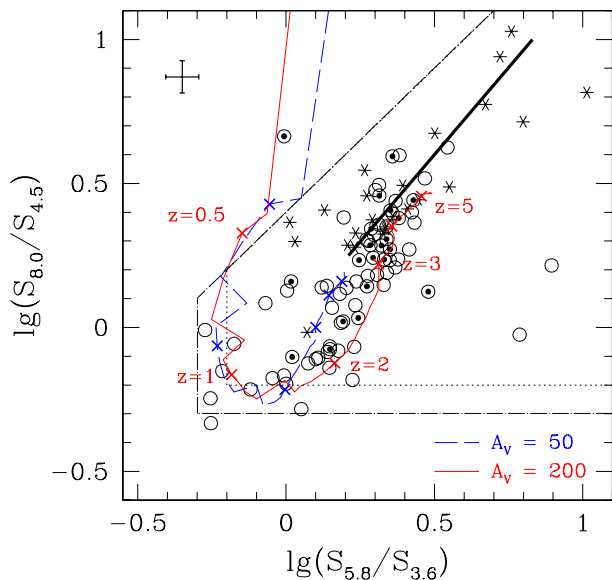
Figure 12. A S_{8.0\mu}/S_{4.5\mu} versus S_{5.8\mu}/S_{3.6\mu} IRAC color diagnostic diagram for heavily obscured starbursts and AGNs based on the color combinations proposed by Lacy et al. (2004). Areas occupied by dusty young starbursts as noted by Yun et al. (2008, see their Fig. 1) are outlined by a dot-dashed line while the area previously identified with power-law spectrum AGNs by Lacy et al. is outlined using a dotted line. The IRAC counterparts identified with the AzTEC sources in GOODS-South and GOODS-North with empty (undetected in X-ray) and dotted circles (detected in X-ray) cluster around the theoretical dusty starburst SED tracks with different amounts of dust extinction ( A_V = 50 & 200 , Efstathiou et al. 2000), as discussed by Yun et al. (2008). The thick solid line represents the theoretical track expected of purely power-law IR AGNs, while asterisks are power-law AGNs reported by Lacy et al. and Martinez-Sansigre et al. (2008). Typical uncertainties in the colors are shown by the cross in the upper left corner.
