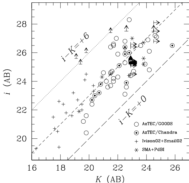
Figure 6. Measured K -band versus i -band magnitudes of the robustly identified AzTEC counterpart sources (circles). Lines of constant color with i - K = +0, +3, \& +6 are shown. Circles with filled dots are AzTEC sources with Chandra X-ray detection in the GOODS-North and GOODS-South fields while empty circles are the sources without X-ray detection. Crosses represent the 17 “securely” identified counterparts to the SCUBA 8-mJy survey (Ivison et al. 2002) and the SCUBA Lens Survey (Smail et al. 2002) sources. Asterisks are SMGs securely identified by interferometric measurements at millimetre and submillimetre wavelengths (Iono et al. 2006; Younger et al. 2007, 2008, 2009; Hatsukade et al. 2010).
