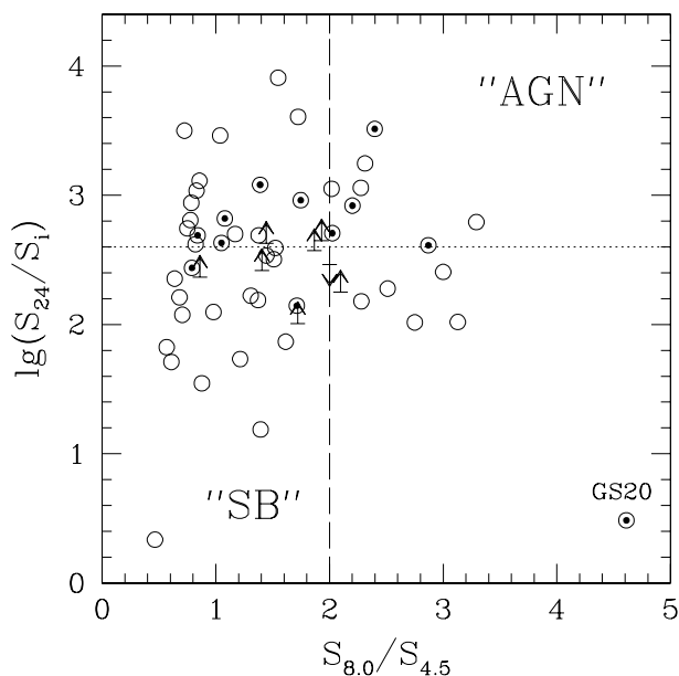
Figure 14. A diagnostic color-color diagram using MIPS 24 \mu\text{m} to optical i -band flux ratio versus S_{8.0\mu}/S_{4.5\mu} IRAC band flux ratio. Symbols are identical to those in Fig. 12. The long-dashed line at S_{8.0}/S_{4.5} = 2 is the dividing line for AGNs and starbursts as proposed by Pope et al. (2008b). The dotted line near \lg(S_{24}/S_i) = 2.6 is the equivalent division line for the z \sim 2 “dust-obscured galaxies” with F_\nu(24\mu\text{m})/F_\nu(R) \gtrsim 1000 – see Dey et al. (2008); Fiore et al. (2008).
