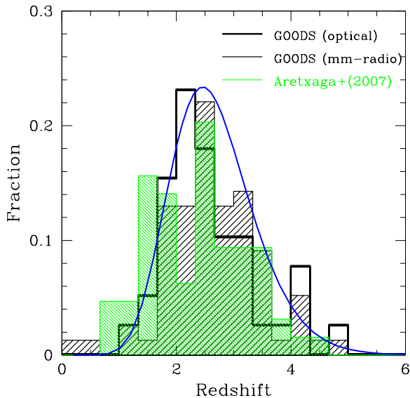
Figure 5. Redshift distribution of AzTEC sources in both GOODS fields based on the optical photoz ( z_{opt} ; blank histogram) and the millimetric photoz ( z_{MR} ; hatched histogram) are compared with that of the 64 robustly detected 850 \mu\text{m} sources in SHADES survey by Aretxaga et al. (2007, shaded histogram). Because of the shallow radio data in the Subaru/XMM Deep Field (SXDF), only the Lockman Hole sources are included for the Aretxaga et al. SHADES redshift distribution. The solid blue curve shown is a log-normal distribution as a function of (1+z) with a mean redshift of z_{\mu} = 2.6 and \sigma = 0.2 .
