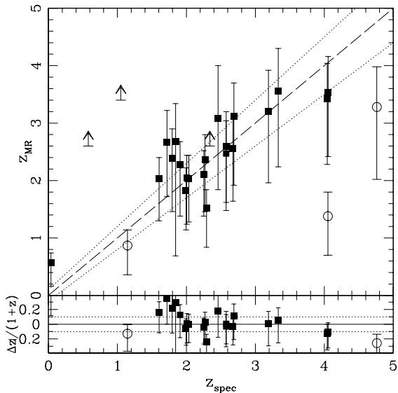
Figure 3. Comparison of spectroscopic and millimeter-to-radio (MR) photometric redshifts for the AzTEC sources with a robust counterpart in the GOODS-South (Table 1) and GOODS-North (Chapin et al. 2009) fields. Three objects with clear evidence for AGN activity are identified as empty circles. The two dotted curves represent redshift uncertainties of \Delta z/(1+z) = 0.10 . The distribution of \Delta z/(1+z) is shown as a function of z in the bottom panel.
