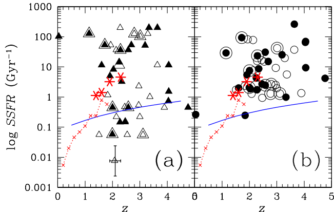
Figure 11. Specific star formation rate of AzTEC counterpart candidates derived from the (a) rest-frame UV and optical SED fitting and (b) far-IR SED fitting using Efstathiou et al. (2000) dusty starburst SED templates. Solid and empty symbols represent the sources with spectroscopic and photometric redshifts, respectively, and those detected by Chandra in the X-ray are identified with a larger symbol. A typical uncertainty is shown for one of the photo- z sources at the bottom of the left panel. The asterisks represent the radio-derived SSFRs for star forming galaxies with M_* \sim 3 \times 10^{10} M_\odot derived by Pannella et al. (2009). The solid line represents the inverse of the Hubble time, and sources above this line are in a starburst mode. The dotted line connecting the crosses represents the average SSFR for massive galaxies with M_* \geq 10^{11} M_\odot found by Damen et al. (2009).
