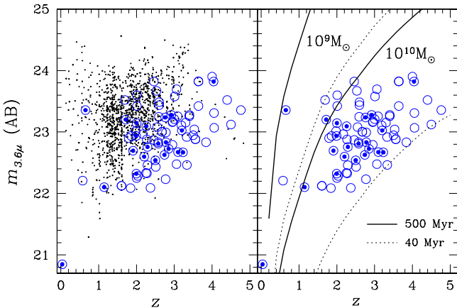
Figure 7. Spitzer IRAC 3.6 \mu\text{m} band “Hubble diagram”. IRAC 3.6 \mu\text{m} band brightness ( m_{3.6\mu} ) of the robust AzTEC counterparts is plotted as a function of redshift. Symbols are the same as in Fig. 6. Small dots on the left panel are K -band selected star forming galaxies with known spectroscopic redshifts in both GOODS fields. The apparent brightness of a 40 Myr starburst population with a stellar mass of 10^9 and 10^{10} M_{\odot} is shown in dotted lines, while the same population after passively evolving for 500 Myr is shown in solid lines. An exponentially decaying starburst history with a 20 Myr e-folding time and solar metallicity is assumed for the models.
