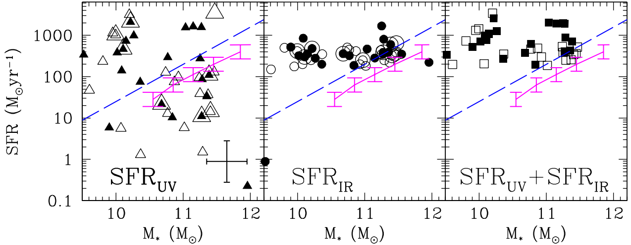
Figure 9. Star formation rates for AzTEC GOODS sources estimated from the rest-frame UV ( SFR_{UV} ) and IR ( SFR_{IR} ) as a function of stellar mass. Open and filled symbols represent photometric and spectroscopic redshifts, and those detected by the Chandra in the X-ray are identified with a larger symbol. A typical overall uncertainty for an object with photoz is shown on the bottom right corner of the left panel. The mean SFR - M_* relation for the z = 2.5 model SMGs fueled by cold flow (Davé et al. 2010) is shown by a solid line. Long-dashed line is the observed mean SFR - M_* relation for the K -band selected galaxies (Daddi et al. 2007). The SMGs do not seem to follow either trends.
