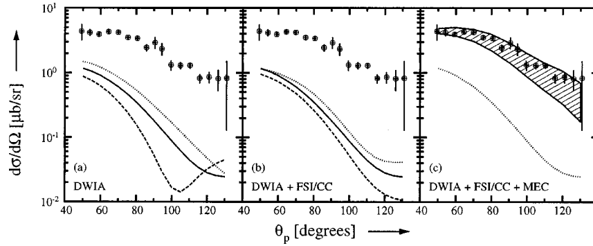
FIG. 2. DWIA calculations compared to the ^{10}\text{B}(\gamma, p_0)^9\text{Be} results at E_\gamma = 56.7 MeV, which are repeated in graphs (a), (b), and (c), subject to varying the ingredients of the calculations: (a) basic DWIA calculation (dashed line), adding orthogonality and antisymmetrization (solid line), and recoil effects in addition (dotted line); (b) DWIA calculation including orthogonality and antisymmetrization using the SOM optical potential (solid line), reduced CC potential (dashed line), or a full CCIA approach (dotted line); (c) DWIA calculation including orthogonality and antisymmetrization using the SOM optical potential with (solid line) and without (dotted line) MEC correction. The hatched area corresponds to the spread introduced in the calculation by the treatment of the FSI's.
