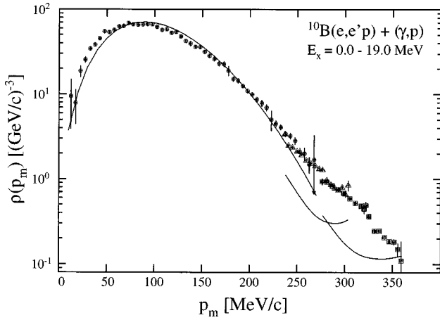
FIG. 5. Reduced cross sections of the ^{10}\text{B}(e, e'p)^9\text{Be} (circles) and ^{10}\text{B}(\gamma, p) reactions [triangles (57.6 MeV) and squares (72.9 MeV)], integrated over the experimentally accessible 1p knockout strength. The solid curves represent DWIA calculations employing the nuclear overlap wave function derived from ^{10}\text{B}(e, e'p)^9\text{Be} data. In the (\gamma, p) case the curves include an incoherent MQD contribution due to two-nucleon knockout.
