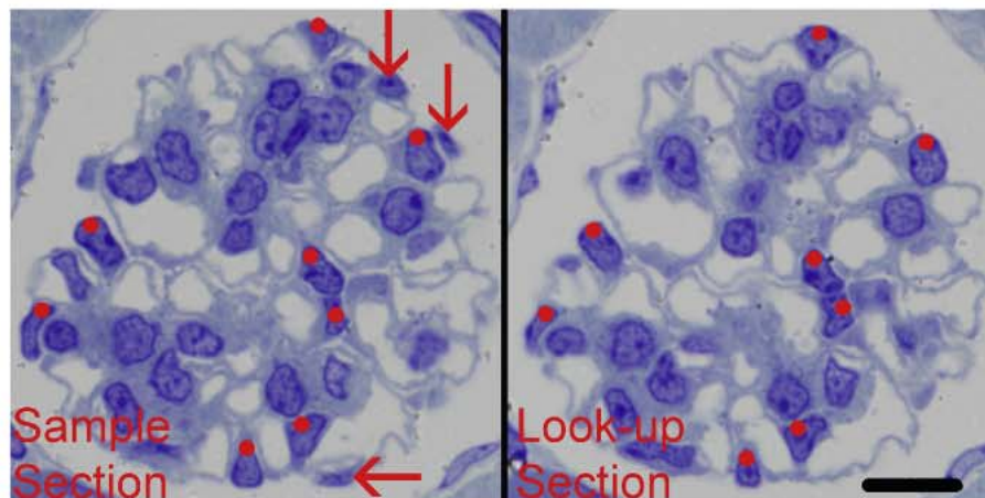
Fig. 1. Disector sections used for counting podocytes. The two images from adjacent 1-mm thick sections formed a disector pair. Profiles from podocyte nuclei present in both sections were not counted (red dots). Profiles from podocyte nuclei present in the sample section but not present in the look-up section (red arrows) were counted as Q^- s and were used to calculate podocyte number. Scale bar = 10 \mu\text{m} .
