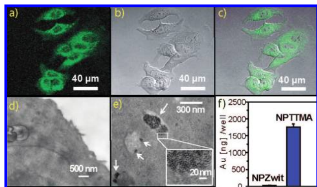
Figure 2. CLSM images of MCF-7 cell treated with AuNPZwit-Bodipy for 2 h: (a) green channel, (b) bright field, and (c) overlap. TEM images of fixed cell treated with (d) AuNPZwit-Bodipy and (e) AuNPZwit-TAF as a positive control. Endosomally trapped AuNPs are marked by arrow. (f) ICP-MS measurement (200 000 cells/well), indicating low cellular uptake of AuNPZwit (31 ng/well after 4 h).
