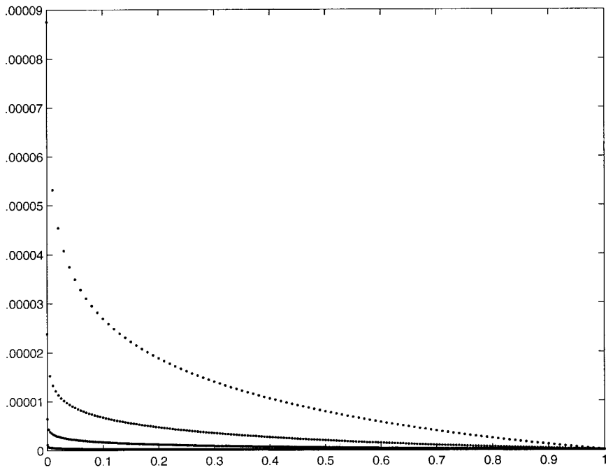
(a) \text{abs}(\text{error}) versus r
