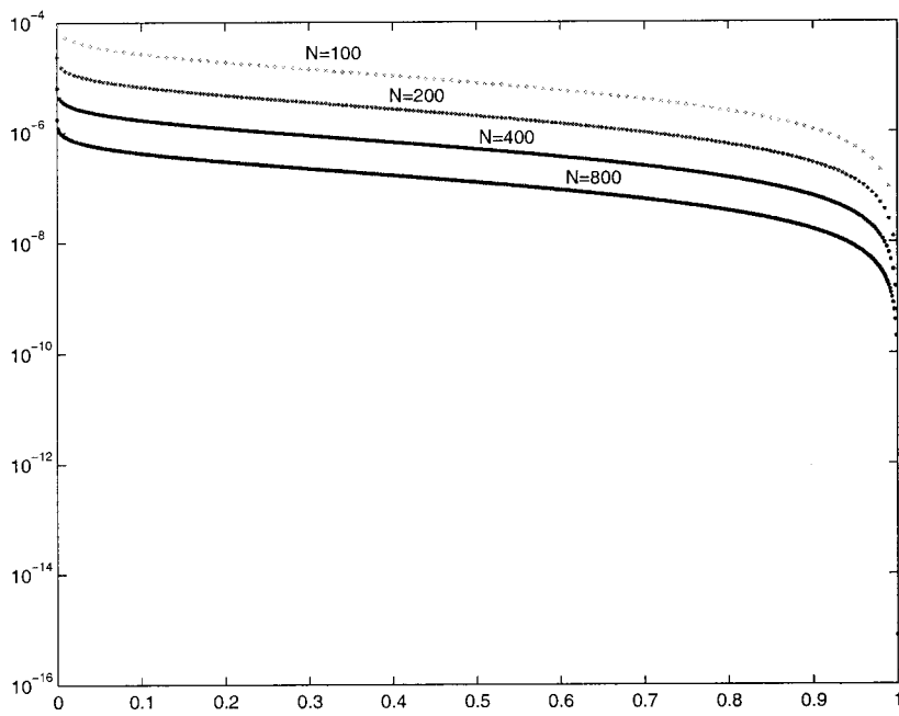
(b) \log(\text{error}) versus r
