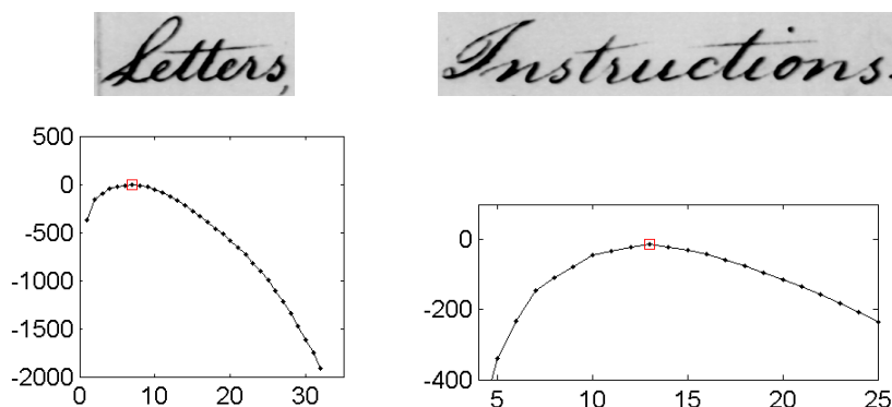
Fig. 5. Mean score per character transition of the best label at various lengths for two sample words. The prediction for the first word is “Letters” and for the second is “Instreictions”. In the latter case, the incorrect 13-letter prediction has higher \hat{\gamma}_m than the correct 12-letter prediction.
