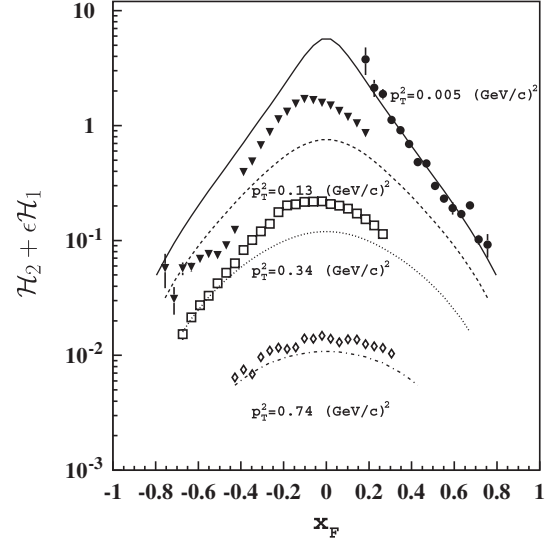
FIG. 25. Same data as in Fig. 24. The curves are the same as in Fig. 24 except for the fragmentation functions, which are evaluated at z_G rather than z .
