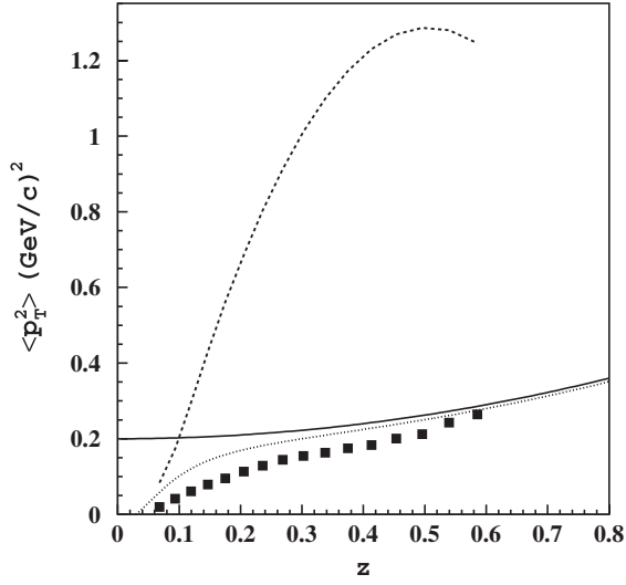
FIG. 15. The z -dependence of \langle p_T^2 \rangle at Q^2 = 2.37 \text{ (GeV}/c)^2 and x = 0.27 . The points are the data from the present analysis. The curves show the maximum allowed p_T^2 = (p_T^2)^{\text{max}} (dashed), the parametrization of high-energy data from Eq. (8) (solid), and the low- z modification from Eq. (23). The error bars are statistical only and they are smaller than the symbol size.
