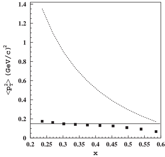
FIG. 16. The x -dependence of \langle p_T^2 \rangle at Q^2 = 2.37 \text{ (GeV}/c)^2 and z = 0.34 . The points are from the present analysis. The curves show p_T^2 = (p_T^2)^{\text{max}} (dashed) and a constant fit to the data (solid). The error bars are statistical only.
