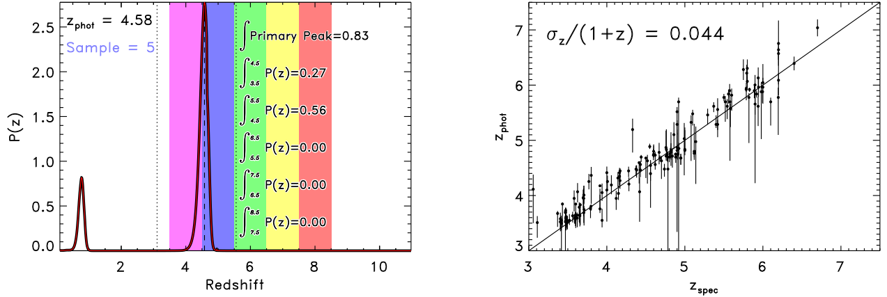
Figure 1. Left) An example of our sample selection. This plot shows the P(z) curve for an object in our z = 5 sample. The best-fit redshift for this object is z_{\text{phot}} = 4.58 , and it contains > 80\% of the area under the P(z) curve in the primary redshift peak. Over 50\% of the area under the P(z) curve falls in the 4.5 < z < 5.5 (i.e., z = 5 ) region, while only \sim 25\% of the area falls in the z = 4 region, thus it is placed in the z = 5 sample. Right) A comparison between the spectroscopic and photometric redshifts for the 157 galaxies in our sample with available spectroscopy. After excluding 12 outliers (not shown), we find excellent agreement, with \sigma_z/(1+z) = 0.044 .
