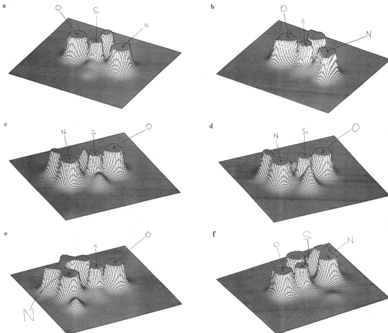
Figure 1. Relief maps of the electron density of silatranes in planes containing Si, N, and O ax atoms. In all figures, the electron density cutoff is set to 0.16 au. All figures are drawn to the same scale and the center of the maps is at the silicon nuclei. (a) n = 0 with electron density generated from 6-31G(d)//AM1; (b) n = 0 with electron density generated from 6-31G(d)//6-31G(d); (c) n = 1 with electron density generated from 6-31G(d)//AM1; (d) n = 1 with electron density generated from 6-31G(d)//6-31G(d); (e) n = 2 with electron density generated from 6-31G(d)//AM1; (f) n = 3 with electron density generated from 6-31G(d)//AM1.
