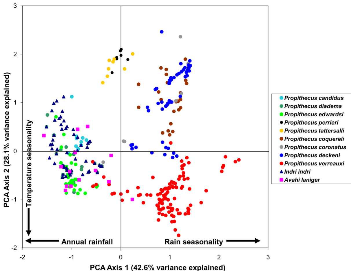
Figure 1. Plot of PCA scores representing the multivariate climatic niche space of Indriidae species based on their known localities. The plot illustrates the same multivariate space as figures 2–5.
