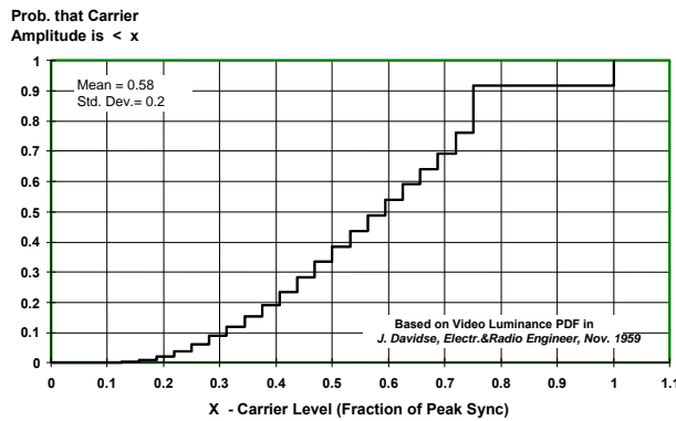
Figure 1. Cumulative probability distribution of RF amplitudes of video modulated NTSC television signal. This function was used for simulating the independent modulation of 75 carriers. The function was constructed based on video luminance distributions provided in Reference [14].
