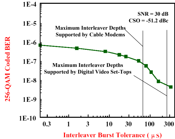
Figure 3. Coded bit error rate of 256 QAM link perturbed by CSO distortion as a function of interleaver burst span. Source of BER results: Ovardia [3].
