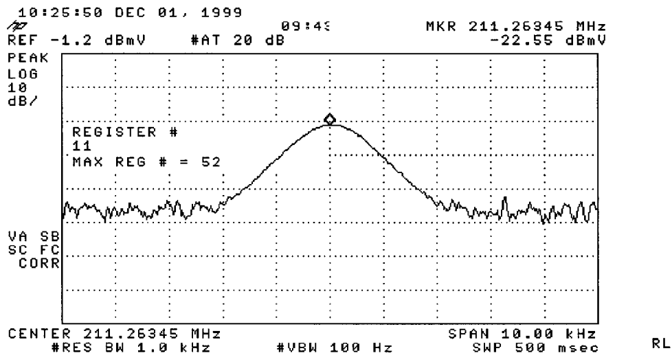
CTB Distortion with a first phase configuration
