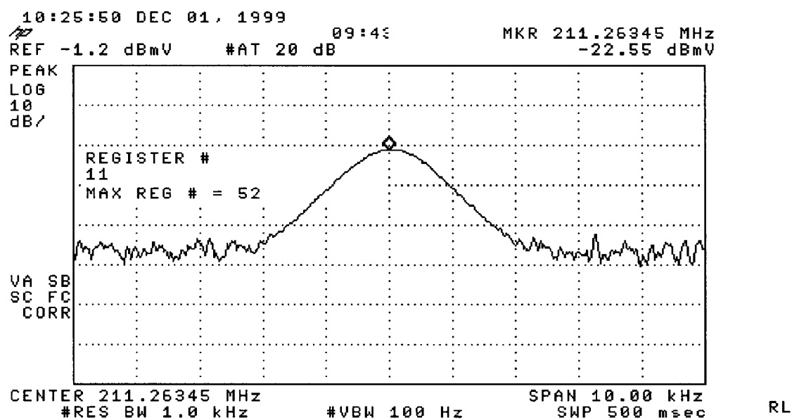
Figure 3 CTB Distortion with a first phase configuration
