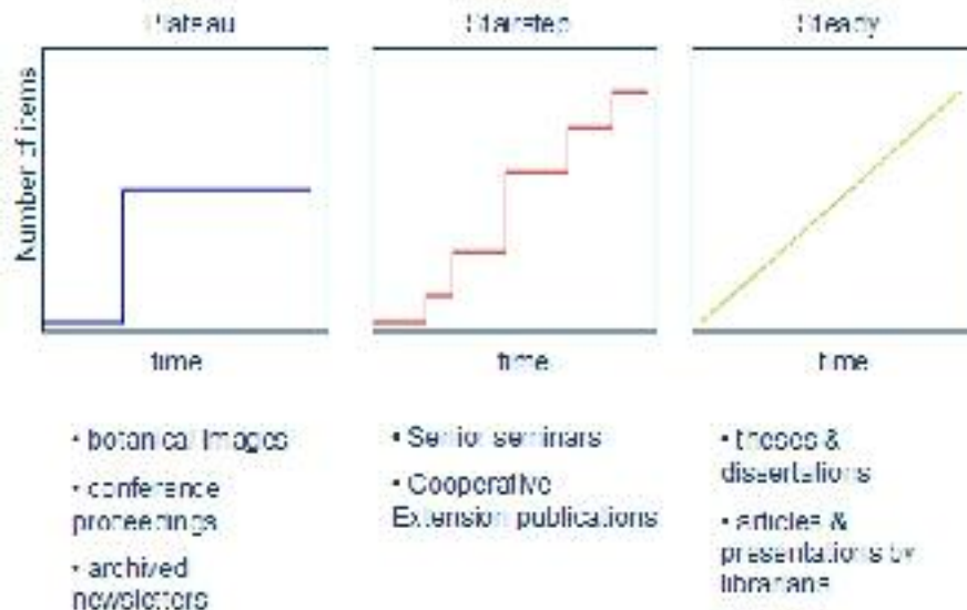
Figure 3. Growth Patterns for DSpace Collections
