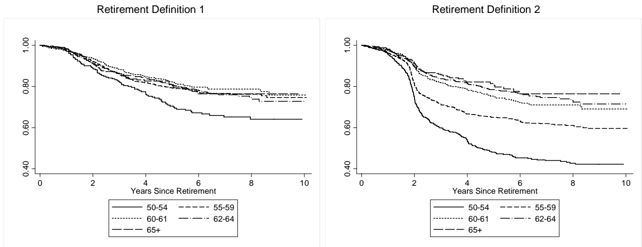
Figure 2. Retirement Survival Curve by Age of First Retirement
