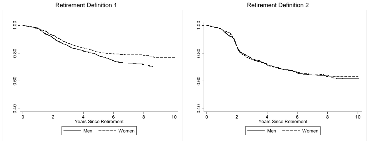
Figure 1. Retirement Survival Curve by Gender
