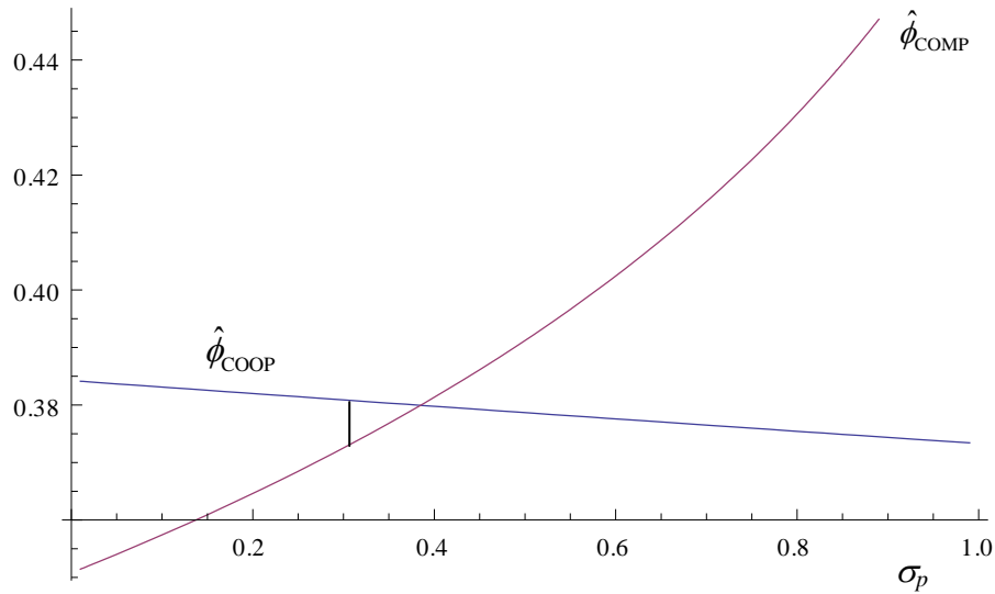
Figure Two ( c(\phi) = \phi^2 , \Pi = 1 , \pi = 0.4 , f = 0.3 , \gamma = 0.5 , \delta = 0.9 , \sigma_i = 0 )
