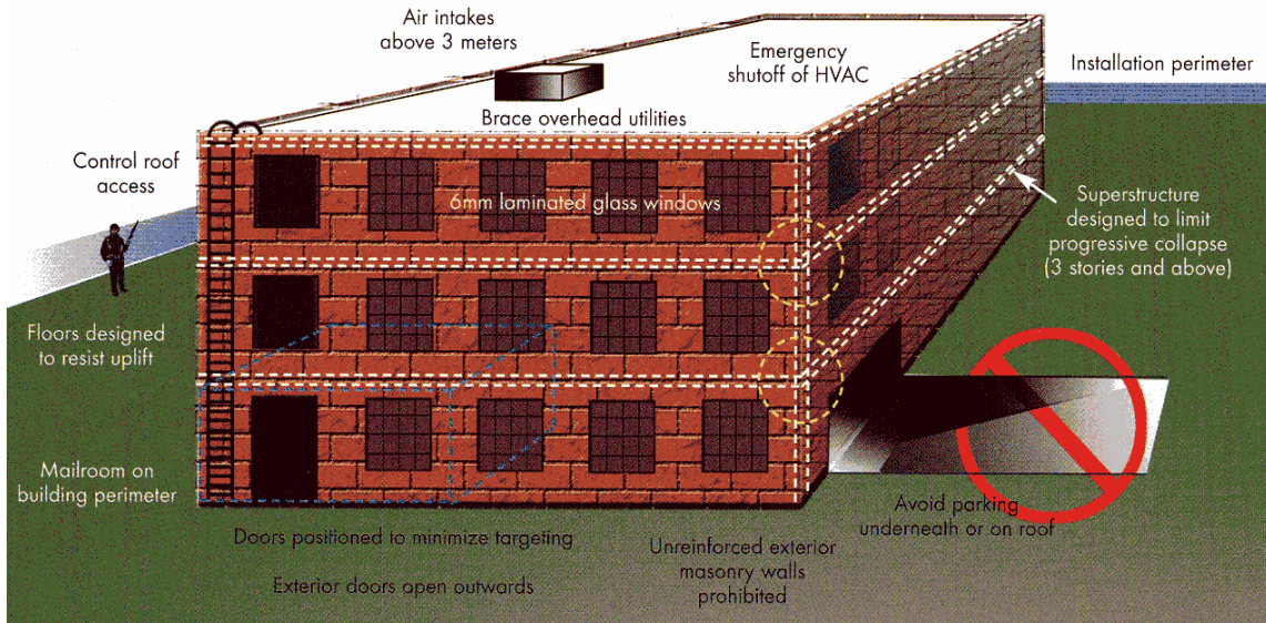
Figure 7. Desired Facility Structural Features 6
