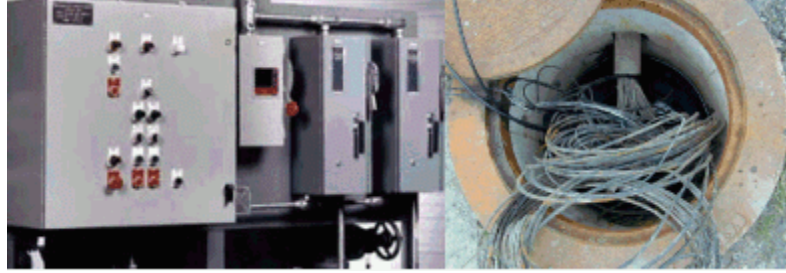
Figure 6. Single Point Failures to Avoid: Commercial/Diesel/UPS in One Electrical Control Panel; Facility Communication Lines Through Single Man Hole
