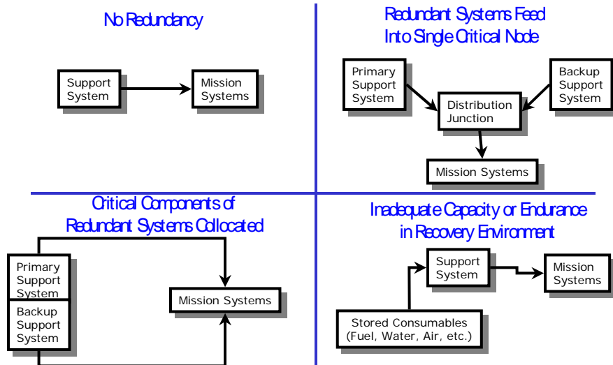
Figure 4. Common Vulnerabilities
