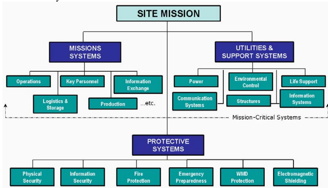
Figure 2. System Taxonomy
