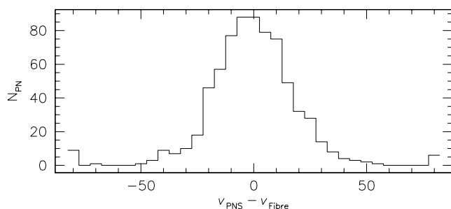
Figure 10. Plot of the difference between final PN.S velocities and H06 fibre-spectrograph velocities. A gaussian fit gives \overline{\Delta v} = -0.7 \pm 0.4 \text{ km s}^{-1} and \sigma = 15.4 \pm 0.4 \text{ km s}^{-1} .
