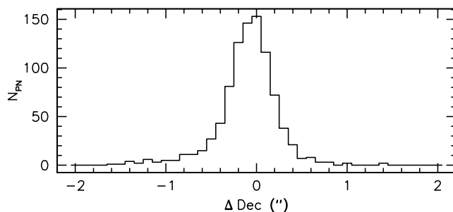
Figure 7. Differences between the positions obtained for repeated observations of PNe in the overlaps between fields. Gaussian fits to these give measurement uncertainties of \sigma_{RA} = 0''.34 and \sigma_{Dec.} = 0''.16 .
